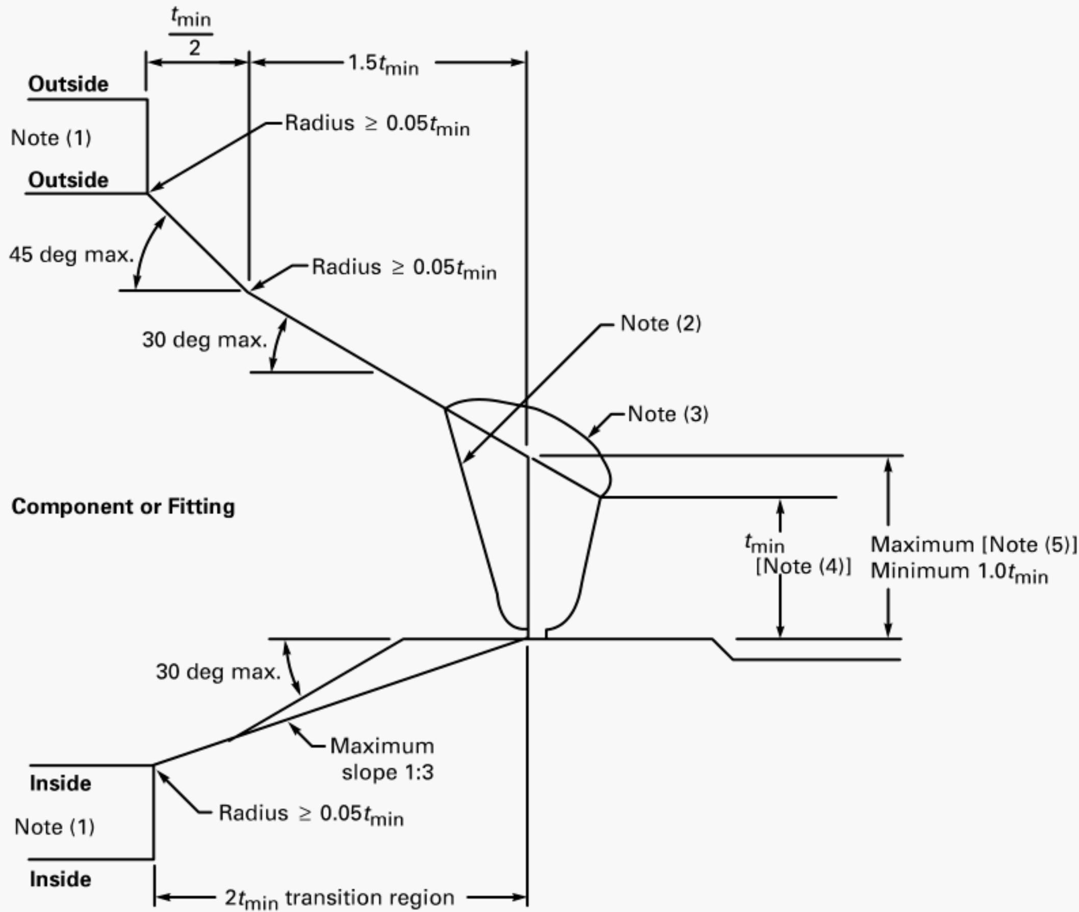
Figure 1 Maximum Envelope for Welding End Transitions
